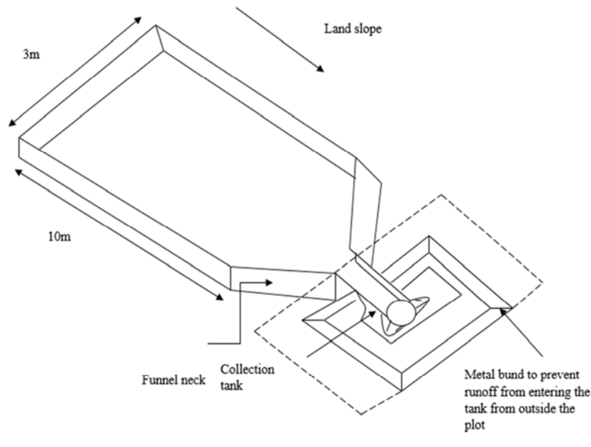
Figure 2. Runoff plot.
