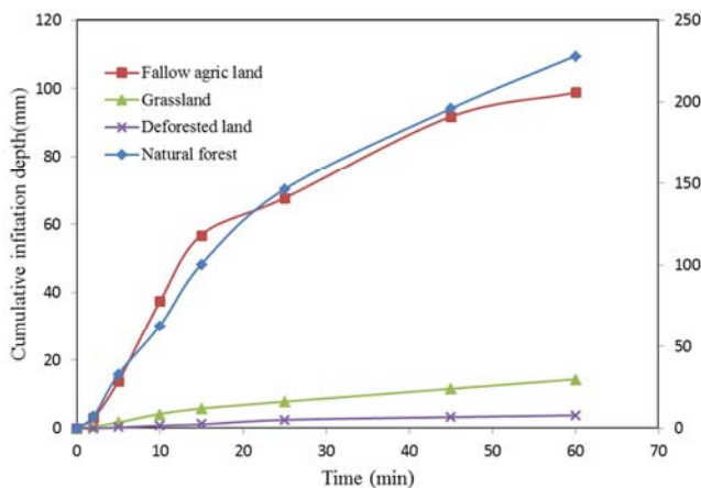
Figure 5. Cumulative infiltration in different land use types.
